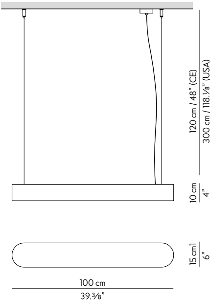
OV.100.17 LED 33W 325mA 2700K 3800lm OV.100.18 LED 33W 325mA 2700K 3800lm
