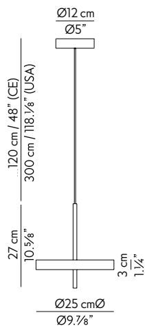
SP.S025.14x LED 14W 24V 2700K 1700lm
