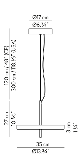
SP.S035.14x LED 20W 24V 2700K 2500lm
