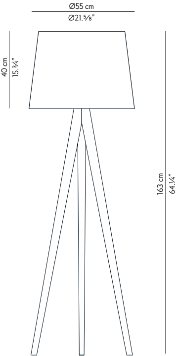
JU.001.00 1 x E27 LED Globe G120 15W
