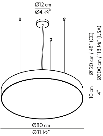
SL.S080.17 LED 66W 325mA 2700K 7600lm IP 20, DALI, Dimmer, Remote, HomeKit
