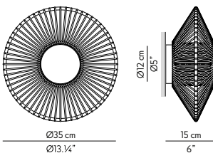
KD.W035.16 LED 8W 230V 2700K 800lm
