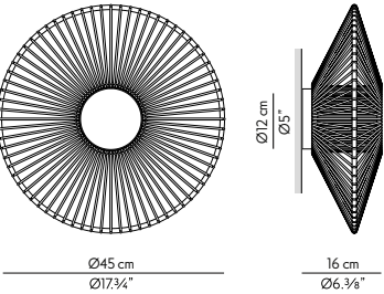
KD.W045.16 LED 8W 230V 2700K 800lm
