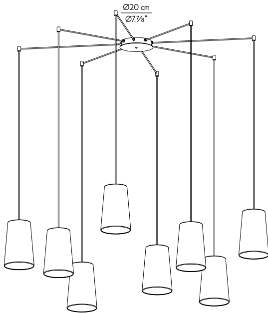
CN.A08.00 8 x E27 LED 12W
