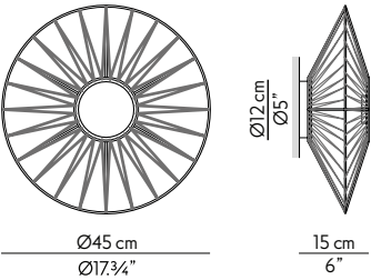
BM.W045.16 LED 8W 230V 2700K 800lm
