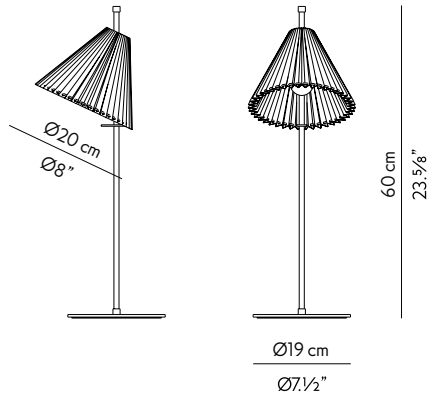
CQ.T020.00x 1 x E14 LED 6W 2700K 800lm
