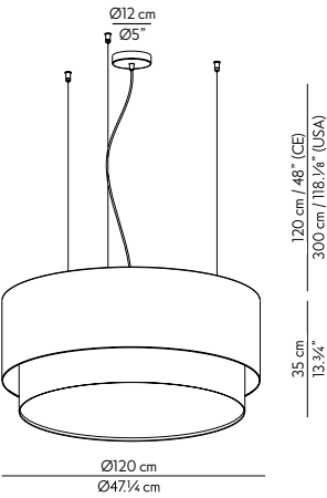
AD.120.00 6 x E27 LED 12W
